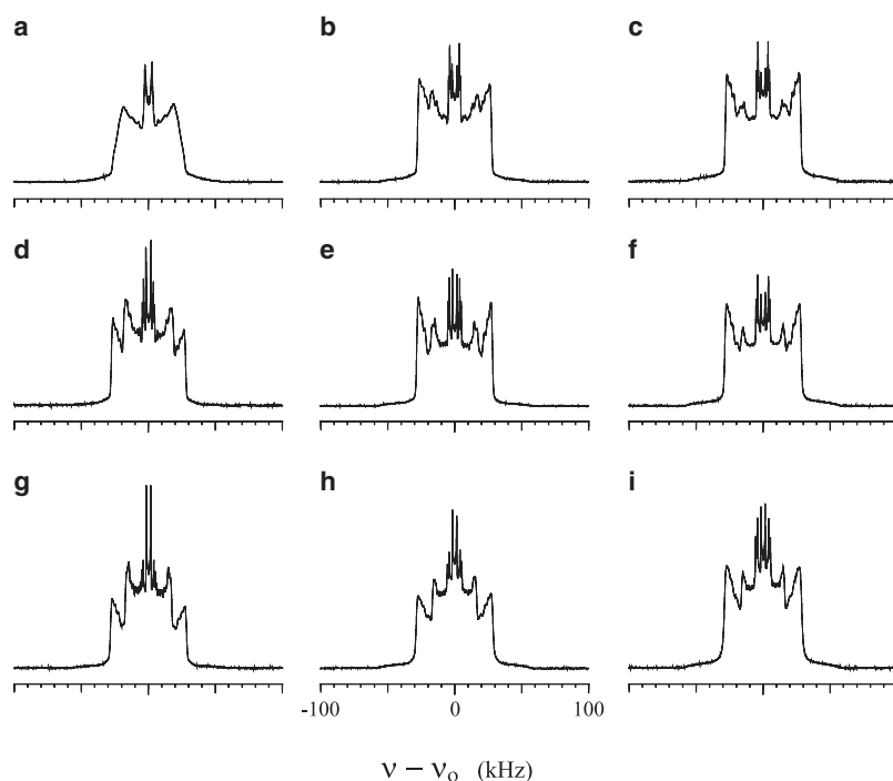
FIGURE 5 ^2\text{H} NMR spectra at 22°C of the same set of sample compositions as in Fig. 4. At this lower temperature, only spectrum a , in the upper left corner, shows evidence of intermediate-timescale averaging.
