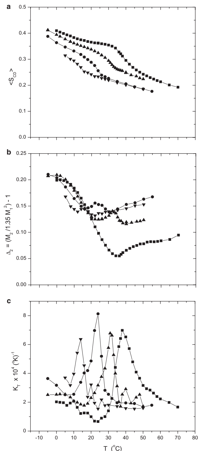
FIGURE 10 Temperature dependence of quantities derived from the moment analysis of the spectra for samples of 25 mol % cholesterol. (a) The average DPPC-d 62 chain C-D bond order parameter, \langle S_{CD} \rangle . (b) The mean-squared width of the distribution of quadrupolar splittings, \Delta_2 . (c) The lipid chain thermal coefficient of area expansion, K_T . Samples were of molar proportions 0:75:25 (squares), 22.5:52.5:25 (upward-pointing triangles), 37.5:37.5:25 (circles), and 52.5:22.5:25 (downward-pointing triangles).
