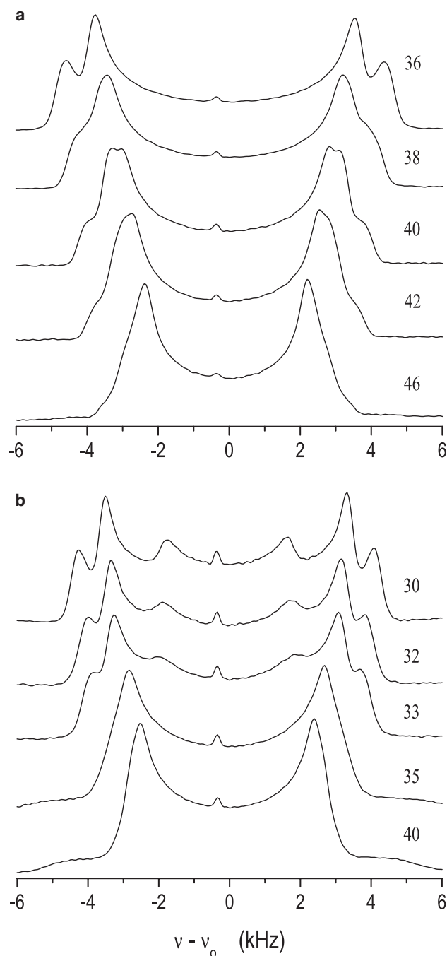
FIGURE 13 Variation of the methyl-group region of the ^2\text{H} NMR spectra with temperature (shown in ^{\circ}\text{C} in the figure) for two different sample DOPC/DPPC- \text{d}_{62} /cholesterol compositions with molar proportions of (a) 0:75:25 and (b) 21:49:30. Both of these examples clearly show the effects of intermediate-timescale averaging at higher temperatures, and two-phase coexistence at temperatures >30^{\circ}\text{C} .
