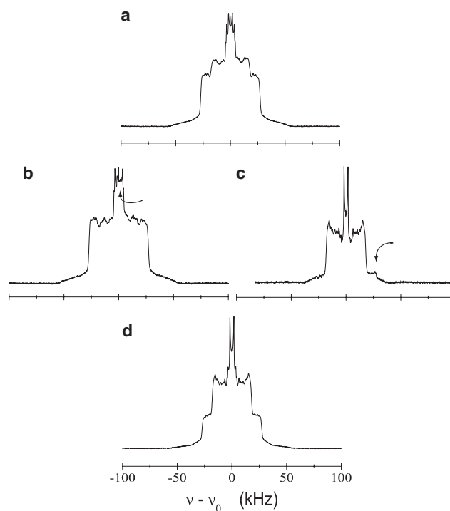
FIGURE 8 ^2\text{H} NMR difference spectroscopy at 28^\circ\text{C} : (a) the spectrum S'_\text{B} of the sample with molar proportions 30:45:25 (normalized area); (b) the spectrum S'_\text{B} - K' times the spectrum S'_\text{A} , with the area of the difference spectrum renormalized; (c) the spectrum S'_\text{A} - K times that in S'_\text{B} , with the area renormalized; and (d) the spectrum S'_\text{A} of the sample with composition 40:40:20 (normalized area). The arrows indicate areas of the \text{l}_\text{d} phase difference spectrum that demonstrate the imperfect subtraction. It is these areas that we attempt to minimize in the subtraction process.
