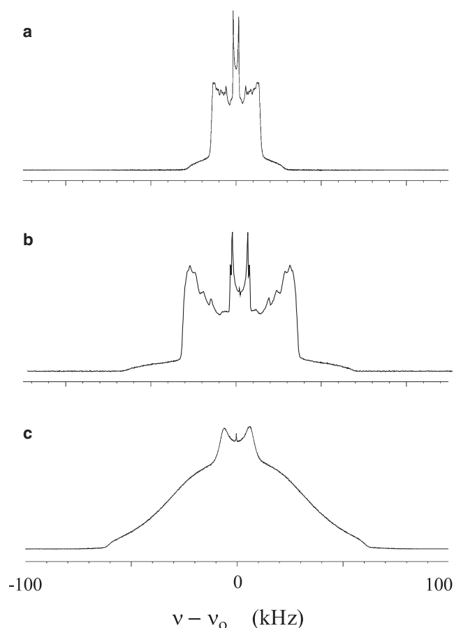
FIGURE 2 ^2\text{H} NMR spectra representative of three phases: (a) typical l_d phase of the DPPC- d_{62} bilayer above 37.75^\circ\text{C} ; (b) l_o phase at 36^\circ\text{C} of DPPC- d_{62} /cholesterol at a molar ratio of 75:25; and (c) gel phase of DPPC- d_{62} below 37.75^\circ\text{C} .
