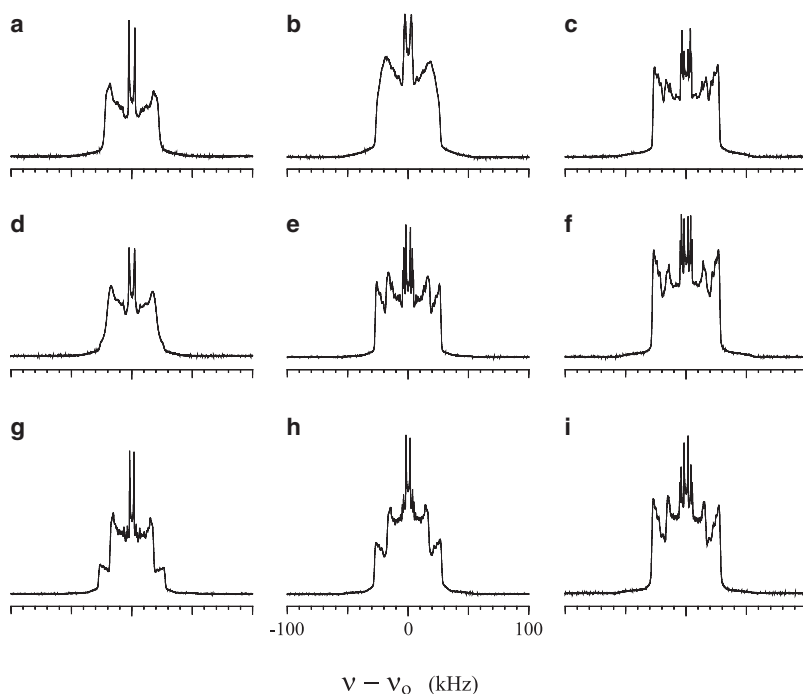
FIGURE 4 ^2H NMR spectra of nine different sample compositions at 26^\circ C . DOPC/DPPC- d_{62} /cholesterol molar proportions: (a) 42:28:30, (b) 35:35:30, (c) 28:42:30, (d) 45:30:25, (e) 37.5:37.5:25, (f) 30:45:25, (g) 48:32:20, (h) 40:40:20, and (i) 32:48:20. The three spectra in the upper left corner (spectra a, b, and d) show evidence of either intermediate exchange between l_d and l_o domains or intermediate-timescale fluctuations in composition.
