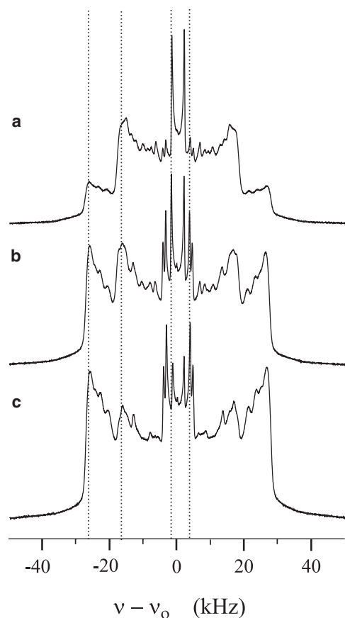
FIGURE 7 ^2\text{H} NMR spectra at 26^\circ\text{C} of DOPC/DPPC- \text{d}_{62} /cholesterol molar proportions of (a) 48:32:20, (b) 37.5:37.5:25, and (c) 28:42:30. The vertical dotted lines are guides to the eye and indicate that each of the principal spectral features occur at nearly the same frequency in all three spectra. These three samples lie close to a common tie-line within the \text{l}_\text{d} - \text{l}_\text{o} two-phase coexistence region in the ternary phase diagram.
